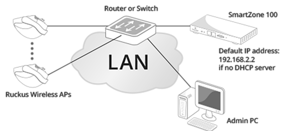
FIGURE 3 Connecting the admin PC, SZ300, and APs to the network
